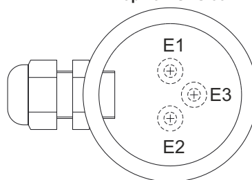
Topview SKS 35
